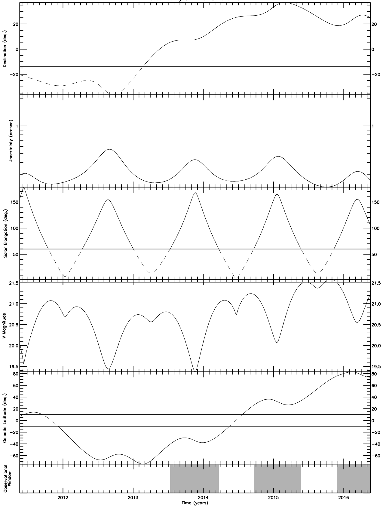
Observability Chart for 2010 GA33
