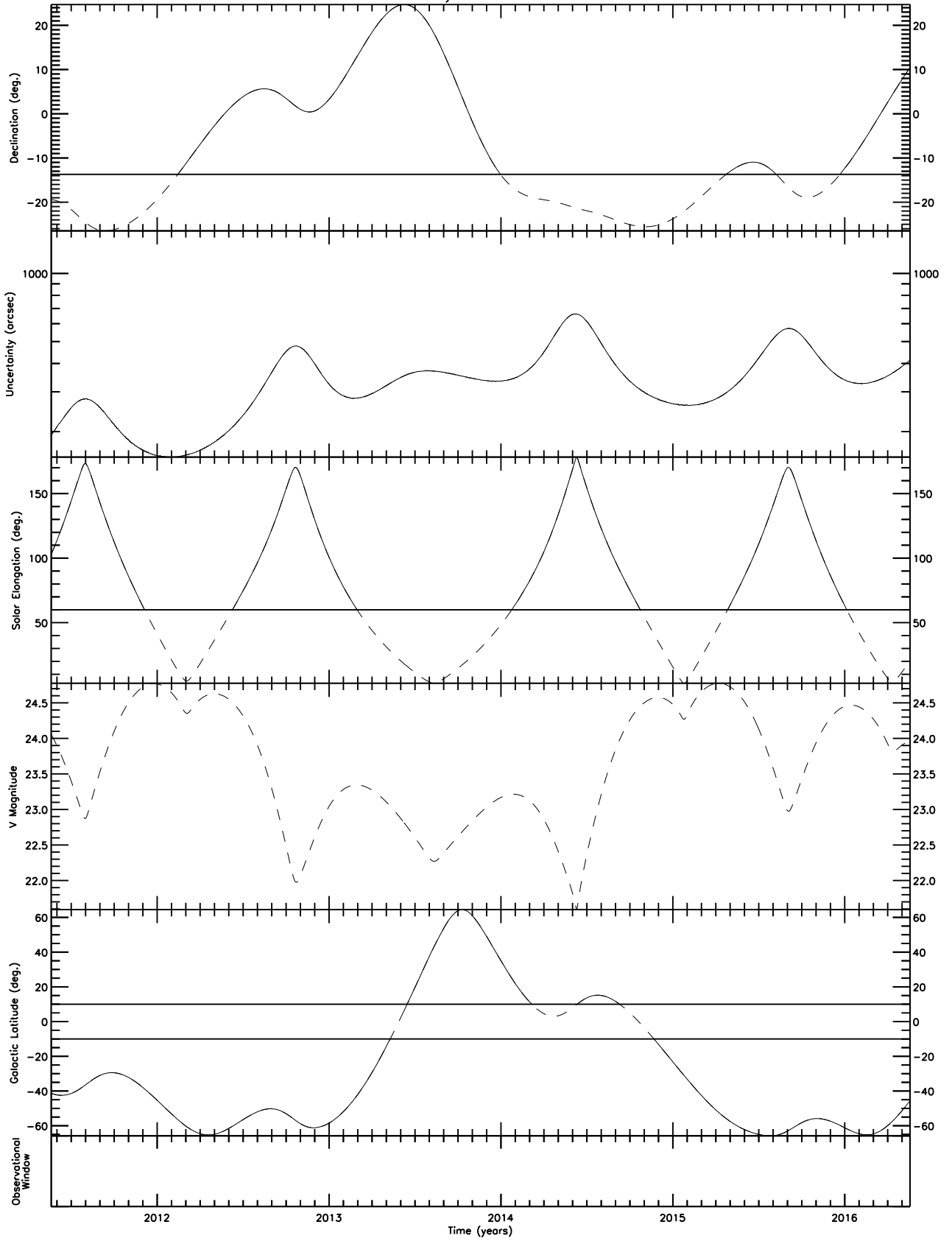
Observability Chart for 2010 DP1
